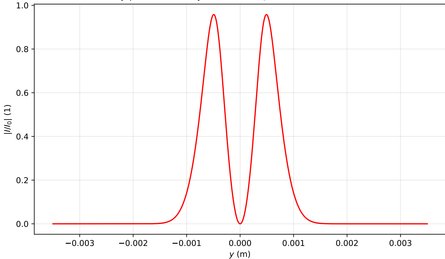
Intensity profile I(x=0, y, z=0.159)/I_0 , \text{Pin}=8.0\text{Pcr} , artificial time
